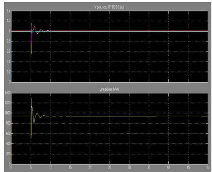
Fig:8 Positive sequence voltage and active power
