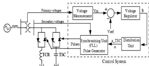
Fig.1.Schematic diagram of SVC [1]
