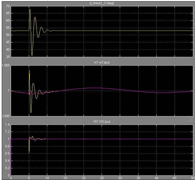
Fig: 9 Rotor angle oscillation of system with controller
