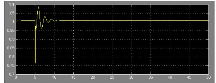
Fig: 7 Terminal voltage of system with svc during LG fault
