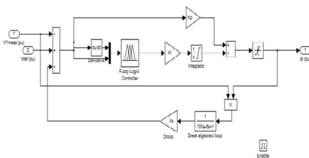
Fig: 6 Subsystem of test model
