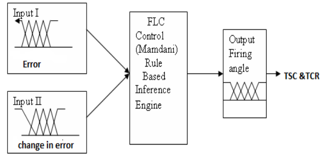
Fig. 2 The structure of fuzzy logic controller
