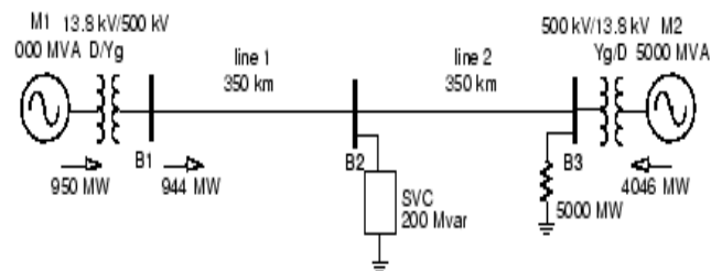
Fig:4 test system line diagramme
