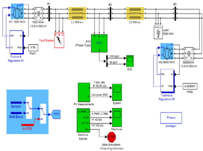
Fig: 5. Two-Machine 3-Bus Test System modeled in Simulink/MATLAB
