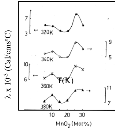
Fig.3 – Variation of thermal conductivity with MnO_2 (mol%) for CuO-MnO_2-B_2O_3 glasses at various temperatures
