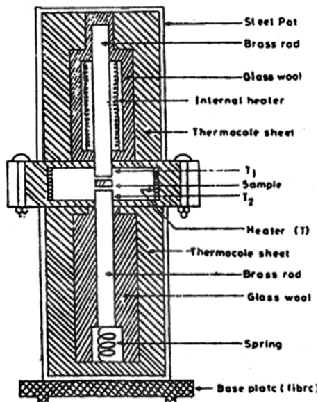
Fig.1-Diagram of apparatus for measurement of thermal conductivity
