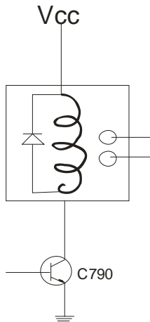
Fig 9: Transistor Relay Driver
