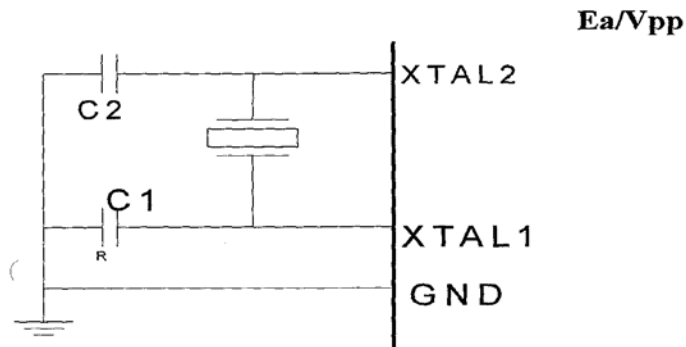
Fig 2: Crystal Oscillator Circuitry
