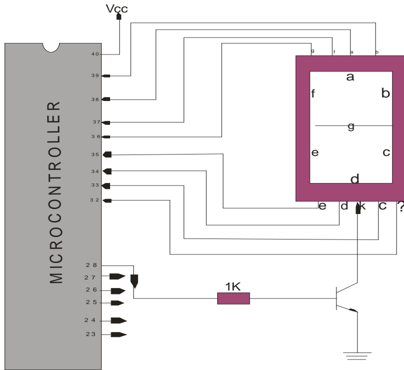
Fig 7: The diagram of 7-segment display interfacing a microcontroller
