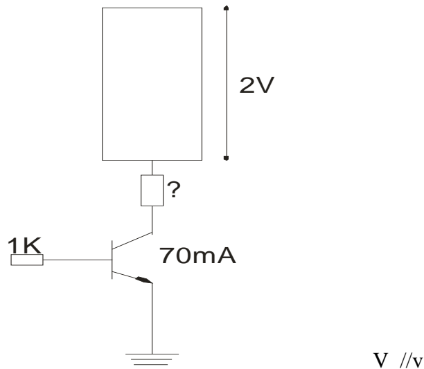
Fig 8: Display connection.
