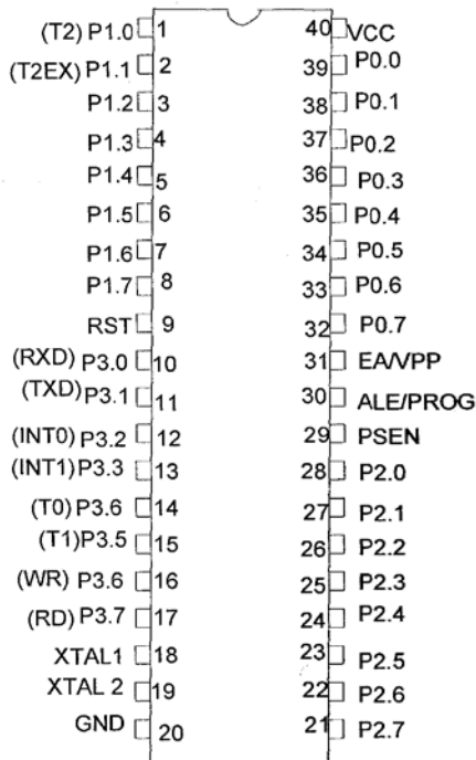
Fig 1: The AT89C52 chip
