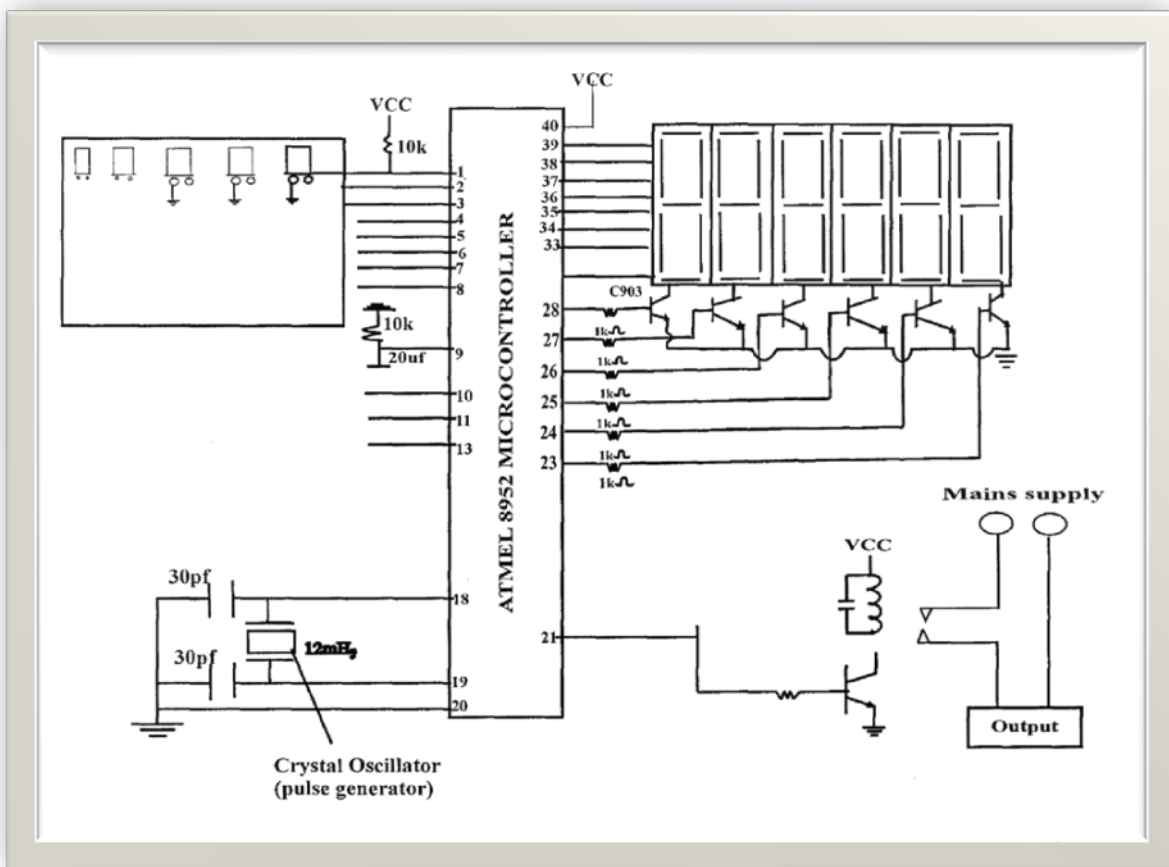
Fig. 4: Circuitry of Power Access Control
