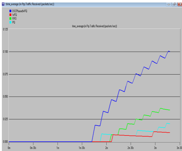
Fig. 10. FTP traffic received (packets/sec)
