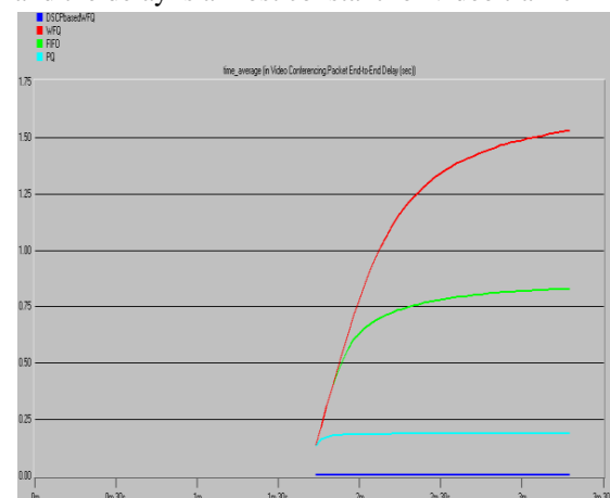
Fig. 9. Video conferencing traffic end-to-end delay (sec)
