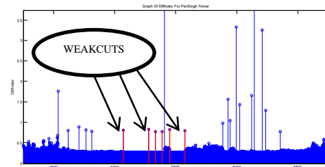
Fig. 4 Difference Index for Weak Cuts
