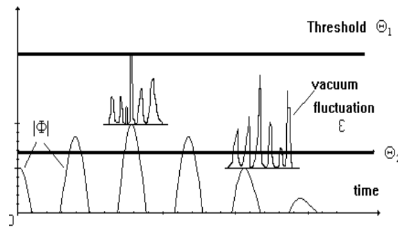
Fig.4. Quantum measurements.
