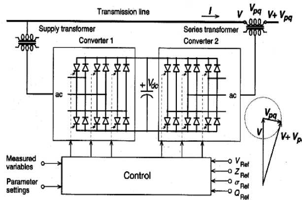
Fig – 3. Unified Power Flow Controller
