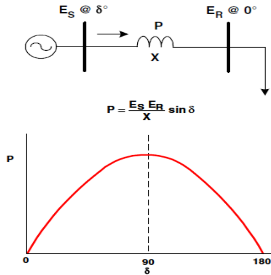
Fig – 2. Illustration of controllability of power systems
