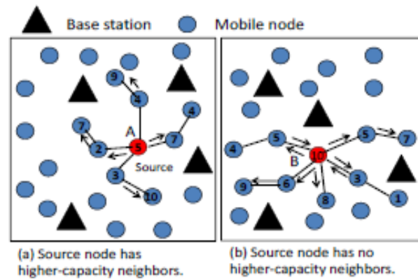
Fig.2: Neighbor node selection process in DTR[1]
