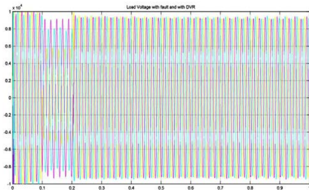
Fig. 13 Waveform of load voltage with line to line fault and with DVR
