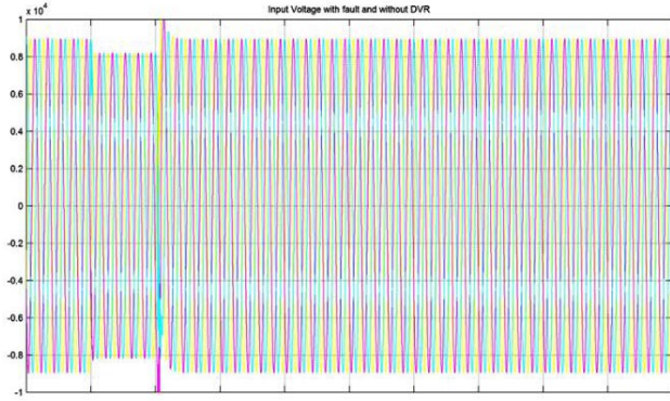
Fig 8 Waveform of input voltage with three phase fault and without DVR
