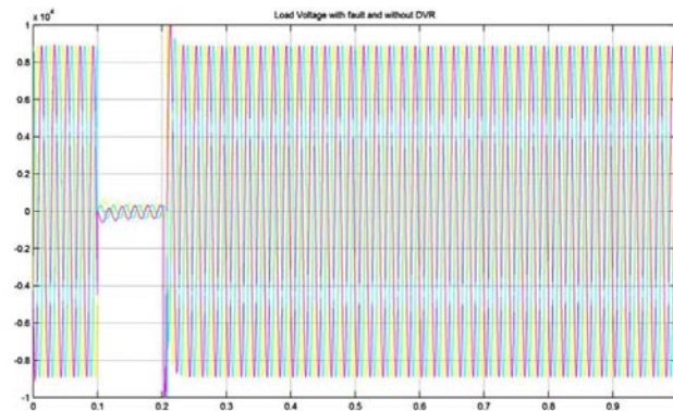
Fig 9 Waveforms of load voltage with three phase fault and without DVR
