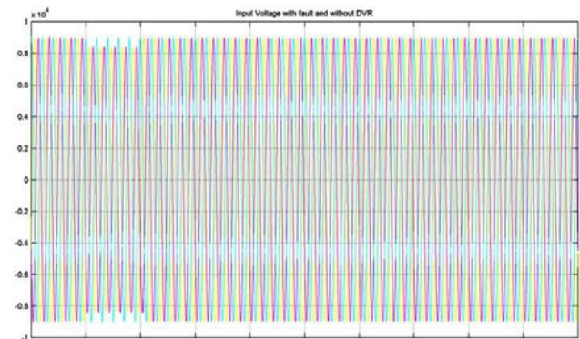
Fig.11 waveforms of input voltage with line to line fault without DVR
