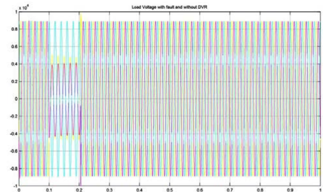
Fig.12 Waveforms of load voltage with line to line fault and without DVR
