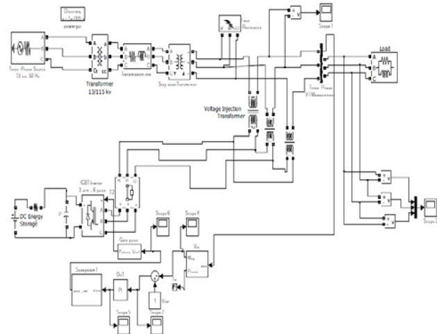
Fig.6 Test model of DVR
