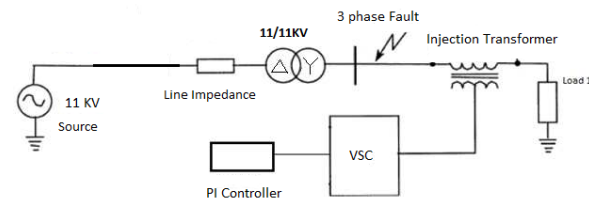
Fig 4: Block diagram of a DVR test model
