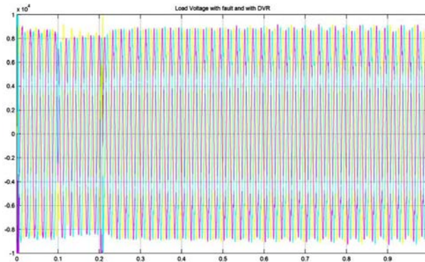
Fig 10 Waveforms of load voltage with three phase fault and with DVR
