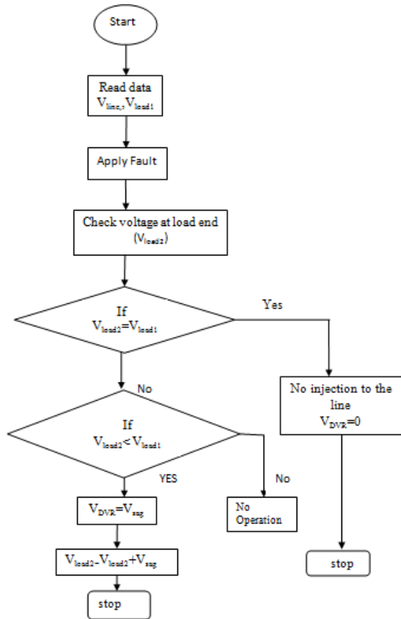
Fig.5 Flow chart of control scheme of DVR
