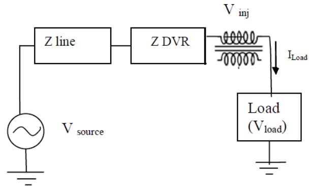
Fig3: equivalent circuit of DVR
