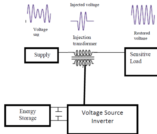
Fig. 1 Operation principle of DVR
