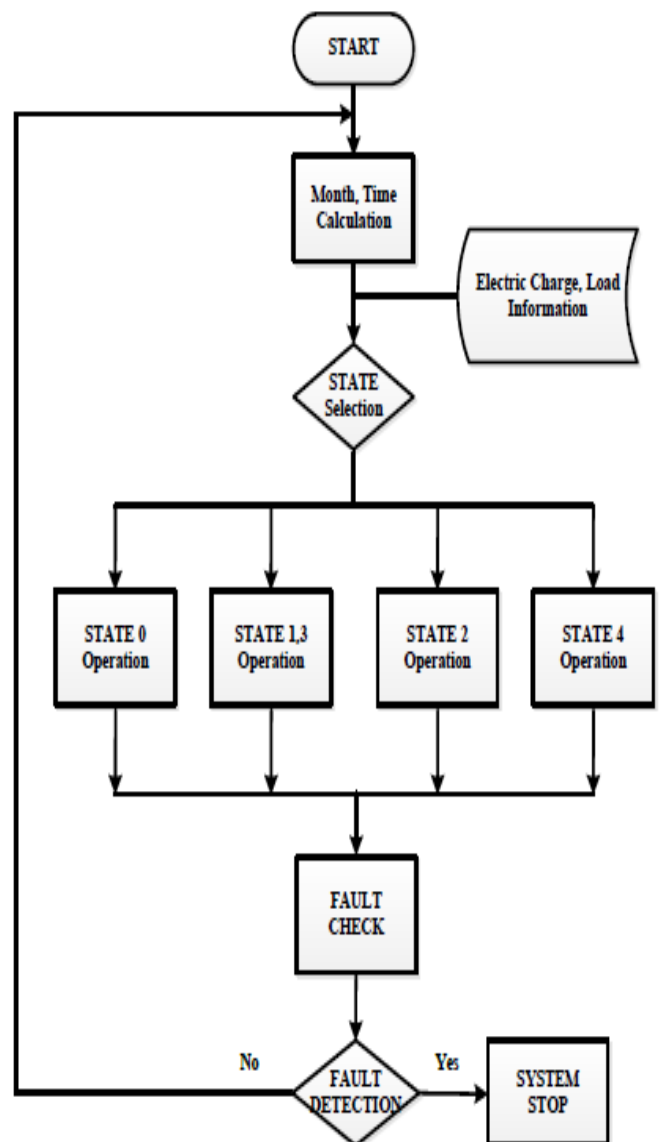
Fig. 7. The operational algorithm of the PV-PPC system.
