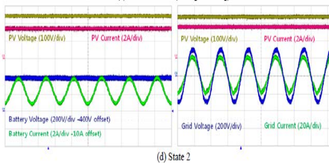
Fig.10. Experiment of the PV-PPC system by state
