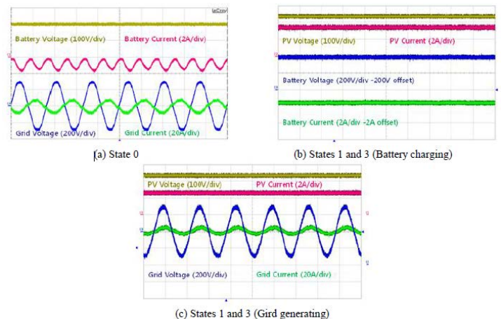
Fig.9 Simulation of PV-PPC system by state
