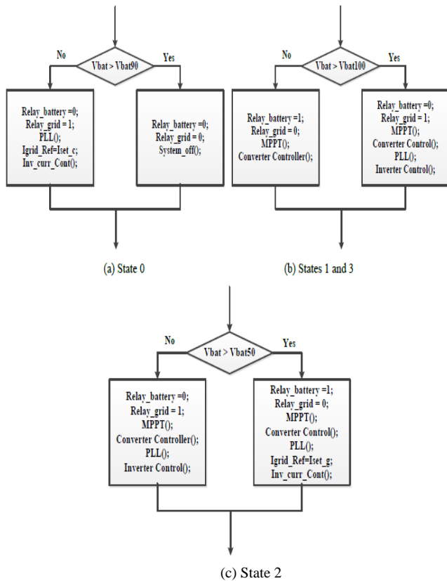
Fig.8. The detailed operation by state
