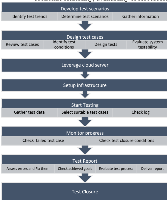
Fig. 4 Overall architecture of proposed testing framework
