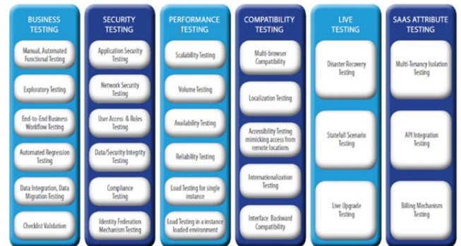
Fig. 1 Features to be tested in cloud application
